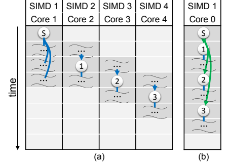
Figure 10: H3 (a) → (b) makes sure small execution groups are not split apart and thus reduces dynamic scheduling overhead.
