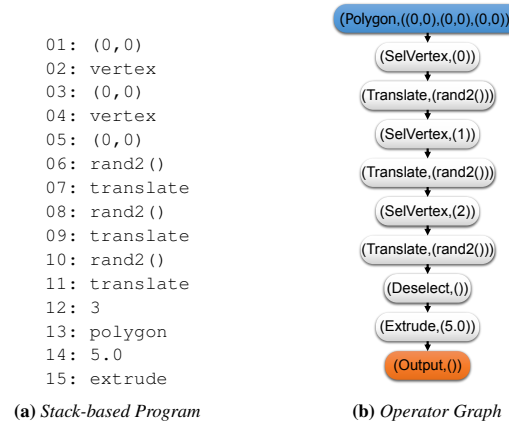
Figure 12: A program written in a stack-based modeling language can be flattened to a data flow graph. As operations used in the operator graph only consume a single object at the time, operations which would require multiple inputs are replaced by a single object and selectors for the sub objects. Note that such a strategy is hardly ever needed in practice.
