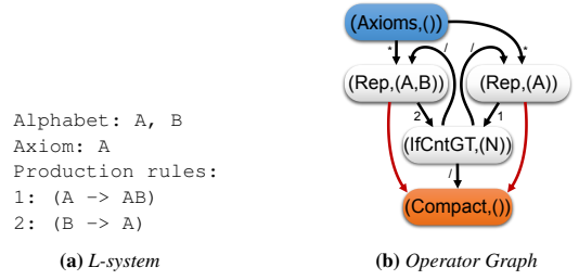
Figure 4: Simple algae L-system and its translation to an operator graph. Red edges indicate dependency edges.
