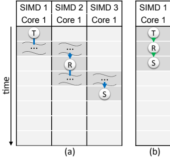
Figure 8: H1 (a) → (b) removes dynamic scheduling if there is only a single object generated.
