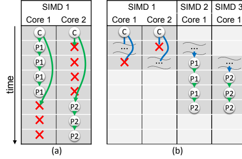
Figure 9: H2 (a) → (b) removes divergence (red crosses) by adding dynamic scheduling under conditional nodes.
